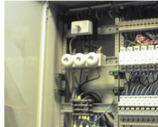
inspecting load problems at electrical cabinets of a public building (police station)
